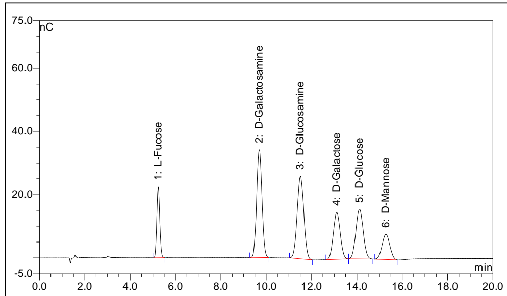
* Example of Monosaccharide Analysis performed on antibody produced in CHO
